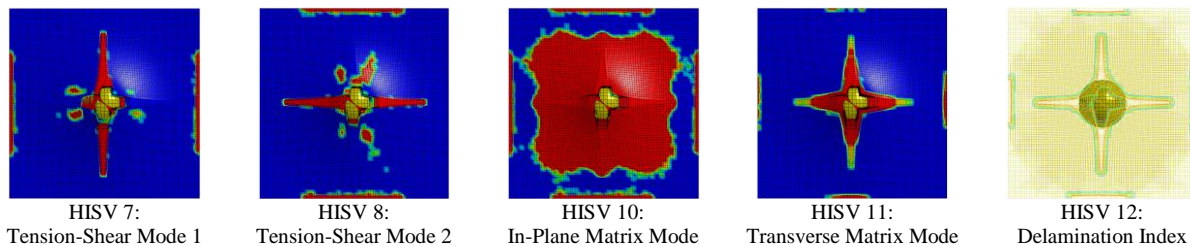
Damage Modes: Solid Elements – MAT162
