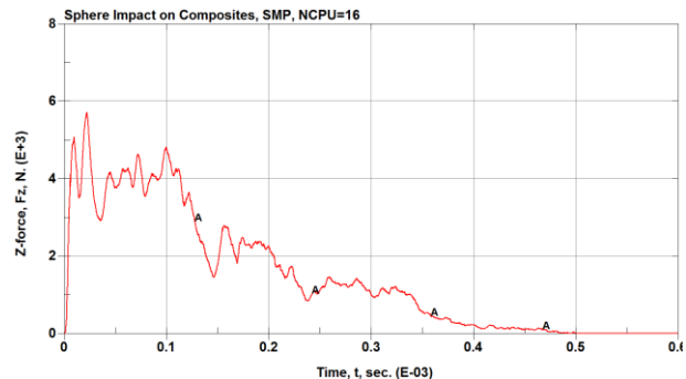
LARGE MODEL with 64000 Elements
