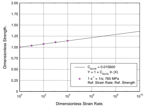
(b) MAT162 Rate Equation for Ref. Strain Rate, \dot{\epsilon}_0 = 1.0 \text{ s}^{-1}
