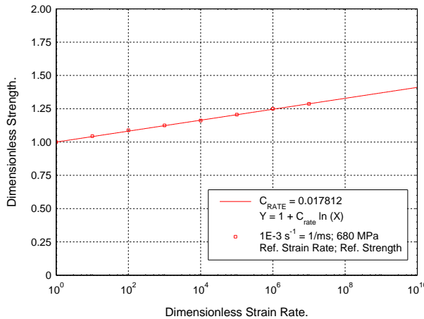
(a) MAT162 Rate Equation for Ref. Strain Rate, \dot{\epsilon}_0 = 1.0 \times 10^{-3} \text{ s}^{-1}
