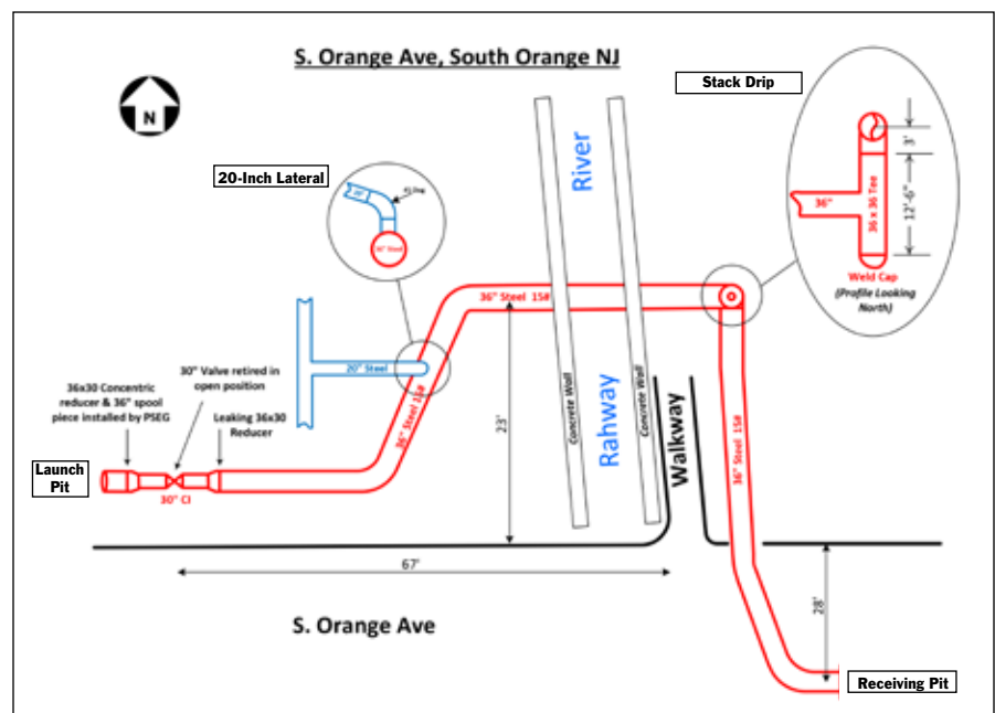
Challenging complex geometry of “The Mess” was compounded and complicated with the dense inaccessible subsurface
