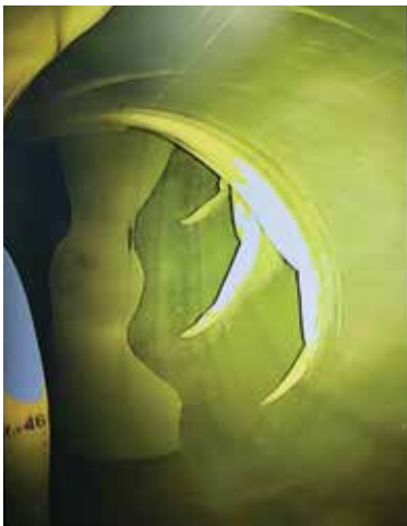
Elbow fabricated from high-strength epoxy was crucial in allowing liner to navigate compound curve with minimal wrinkling
