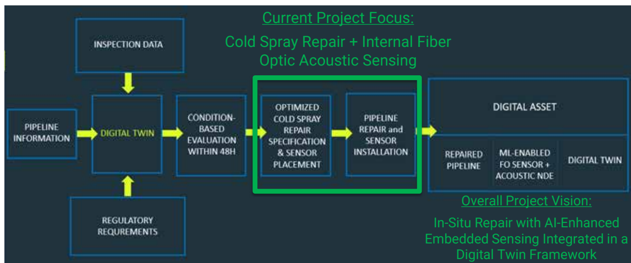
Overall vision of “innervated pipelines”, leveraging fiber optic sensors and AI, combined with cold spray-based metallic repair technology
